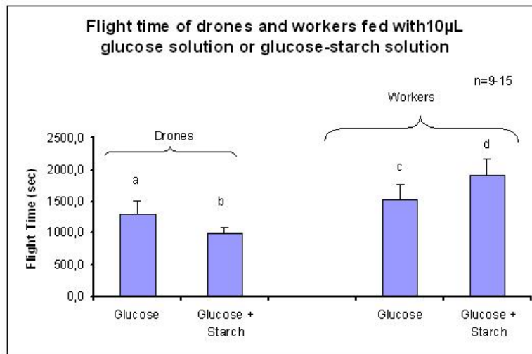
Figure 1 - Total flight time of drones and workers fed either 10 \mu l of a 2 molar glucose solution or 10 \mu l of a 2 molar glucose plus starch solution, which equals a 3 molar glucose solution. Identical letters above columns indicate no statistically significant difference (ANOVA; P < 0.05 )
